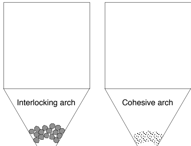
Figure 8. Knowing the characteristics of these two types of flow obstructions will help determine outlet size.
