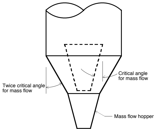
Figure 7. Dashed trapezoidal shape indicates the second hopper inside the existing hopper.
