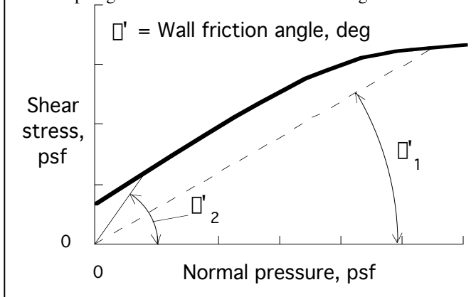
Figure 4. Typical results of the test setup shown in Figure 3 to help engineers determine wall friction angle.
