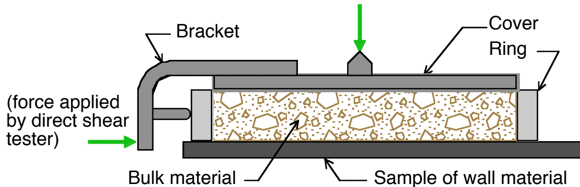
Figure 3. Test setup design allows shear stress (see horizontal arrow) to be measured as a result of applied weights (see vertical downward arrow).
